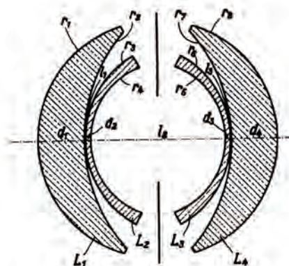
Lens section of the Topogon 4/25 lens
