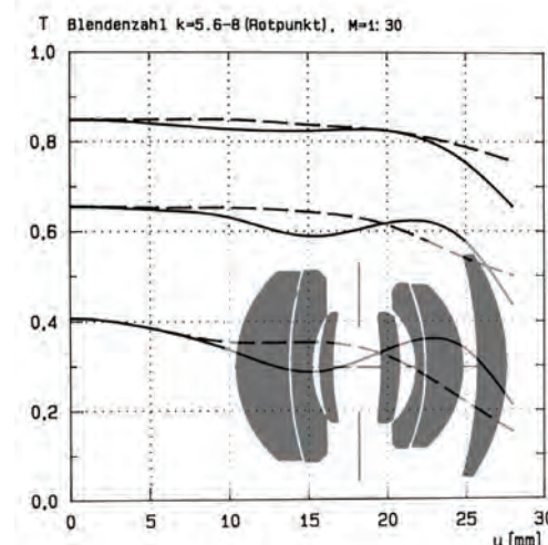
S-Orthoplanar for documentation on microfilm in 32x45mm format; MTF for spatial frequencies of 25, 50 and 100 Lp/mm. The radial distortion is less than 0.1%.
