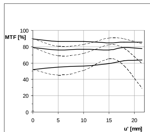
MTF curves of lens B in close-up range with a reproduction scale of 1:10, aperture 2.8 (above) and aperture 5.6
