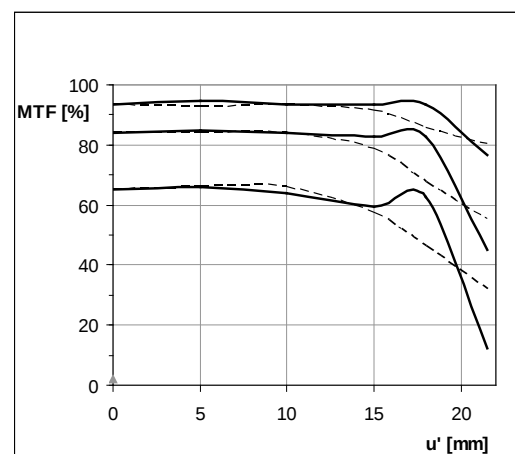
MTF data of the Makro-Planar T* 2/50 at infinity, scale 1:10 and 1:4 (from top to bottom), apertures 5.6 (top) and 4.
