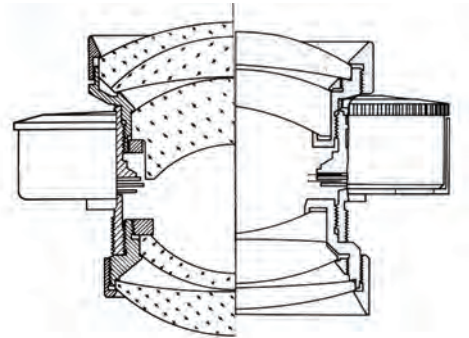
Design of the 5-element Gauss model Planar 2,8/80 (left) and 3.5/75 for the 6x6 format.
